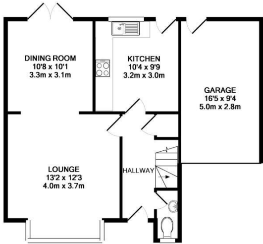
GROUND FLOOR APPROX. FLOOR AREA 633 SQ.FT. (58.8 SQ.M.)
